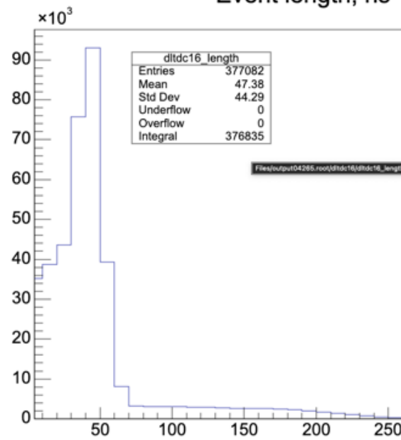
Event length, ns
