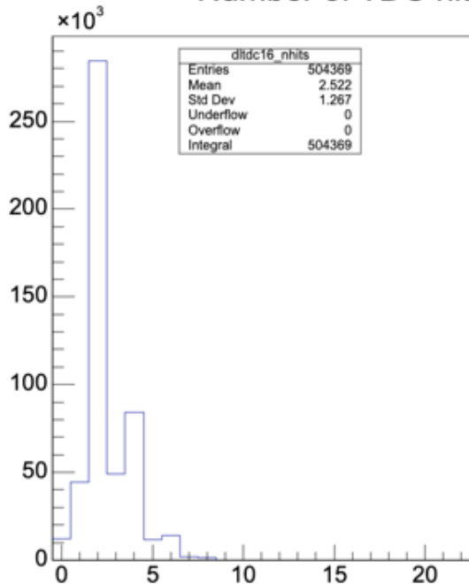
Number of TDC hits
