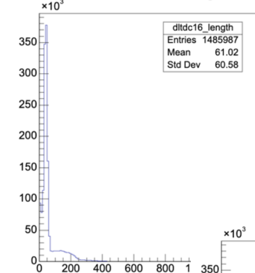
Event length, ns
