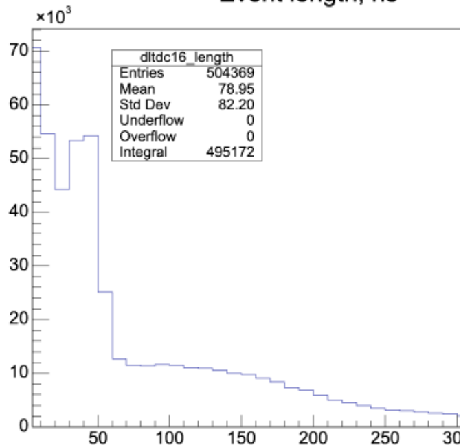
Event length, ns
