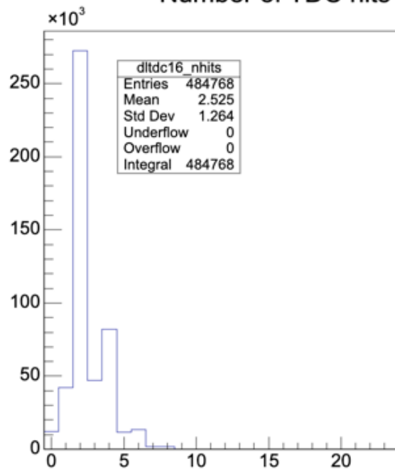
Number of TDC hits
