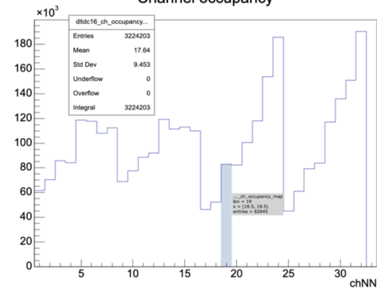
Channel occupancy
