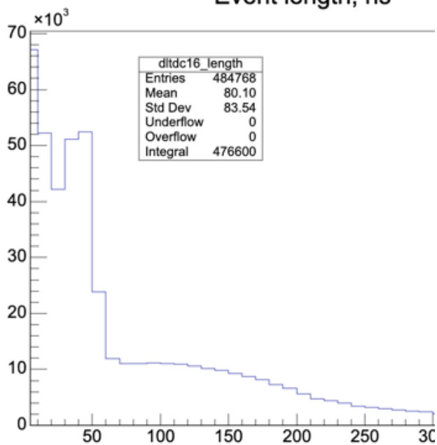
Event length, ns
