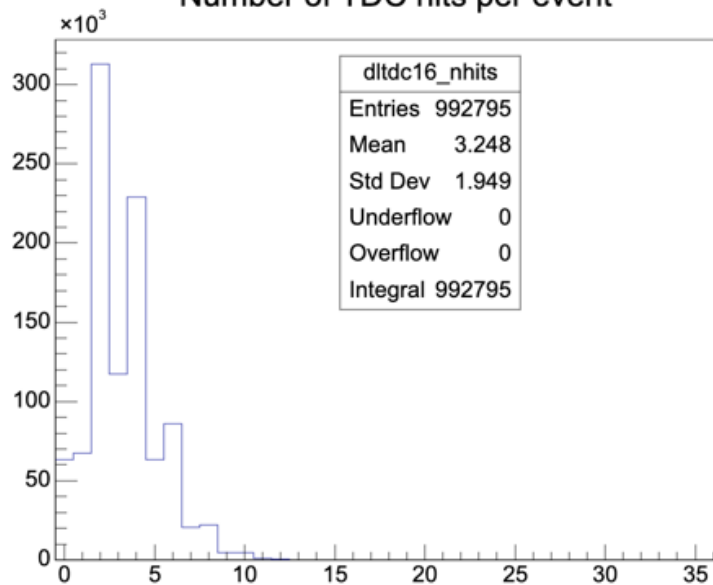
Number of TDC hits per event
