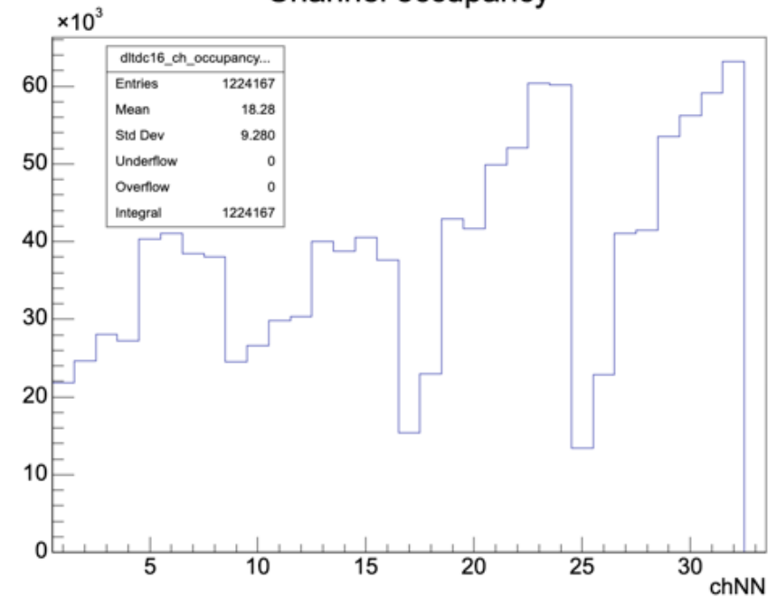
Channel occupancy
