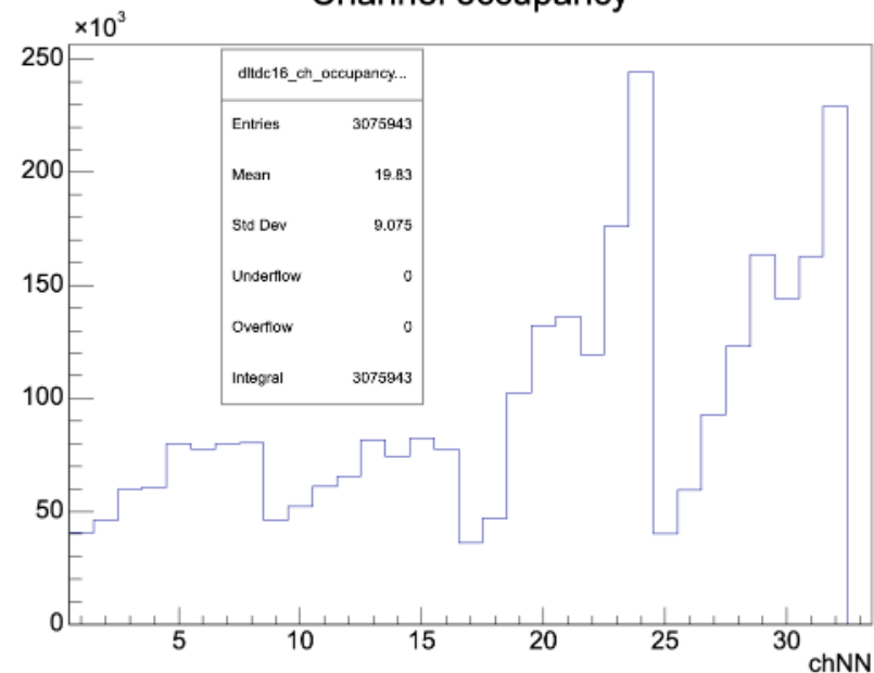
Channel occupancy
