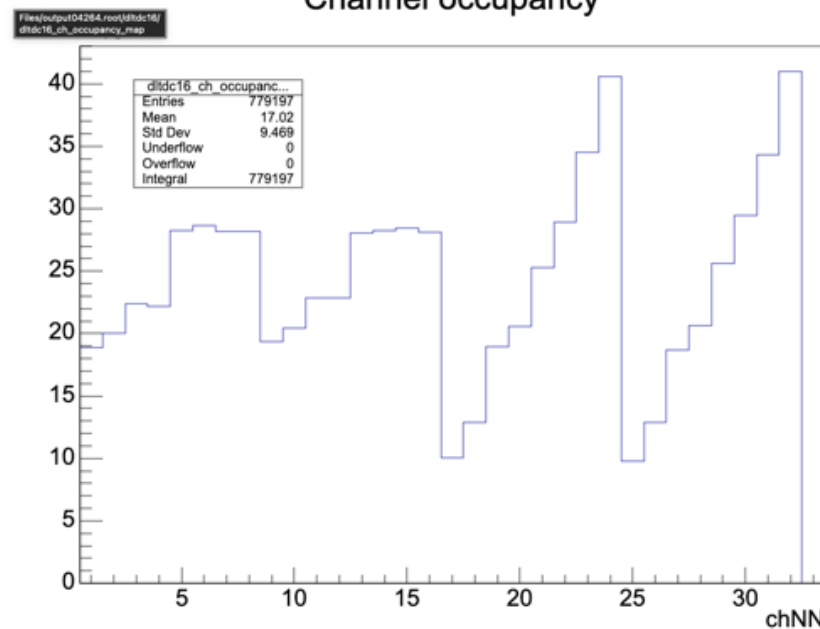
Channel occupancy
