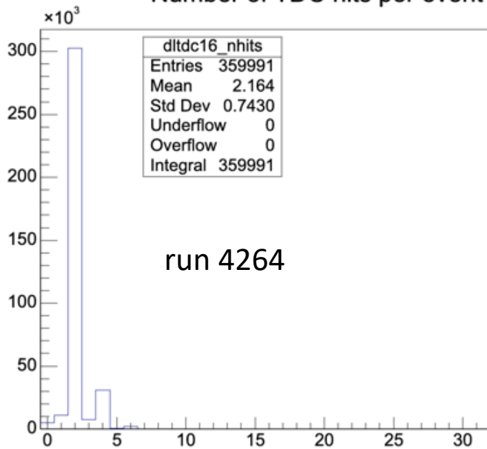
Number of TDC hits per event
