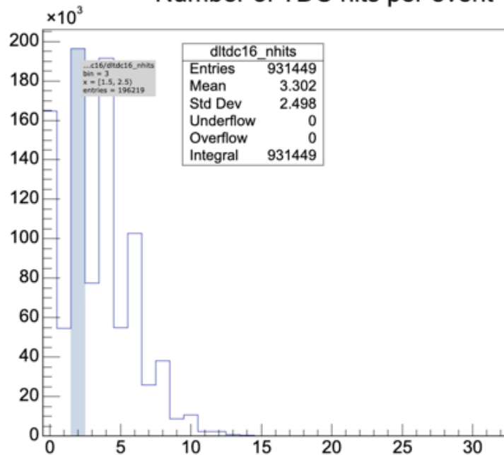
Number of TDC hits per event
